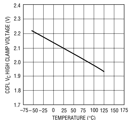
V C High Clamp Voltage vs Temperature
