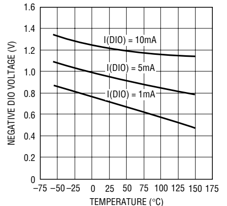
Negative DIO Voltage vs Temperature
